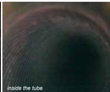
Chiller #3 Condenser Ø 67 cm, tube Ø 7/8", length: 418 cm
